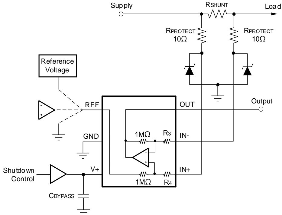
Figure17. RES199 Transient Protection Using Dual Zener Diodes
