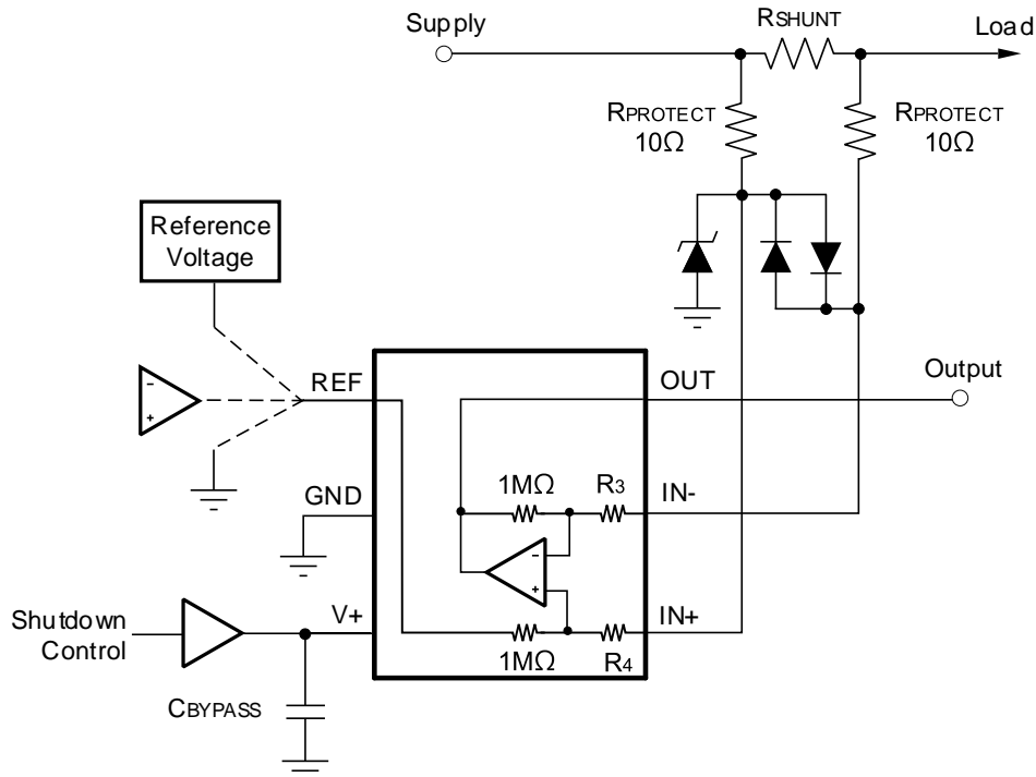
Figure 18. RES199 Transient Protection Using a Single Transzorb and Input Clamps
